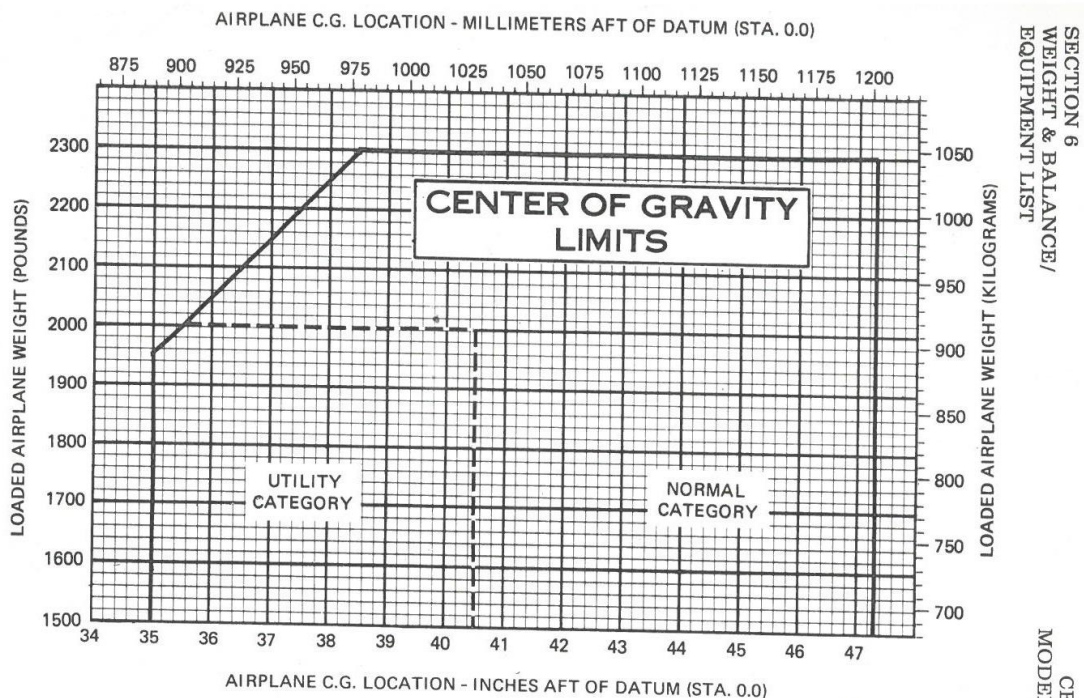
Figure 6-8. Center of Gravity Limits
